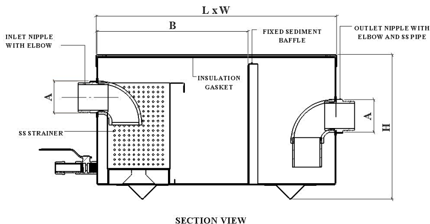
SECTION VIEW
